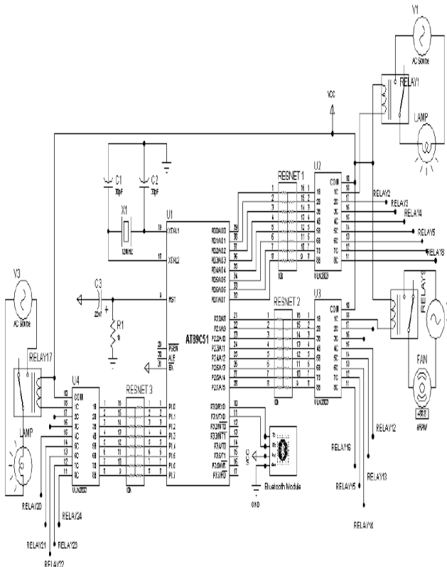
Fig.2. Home authentication circuit.
