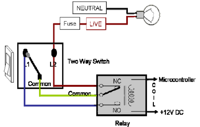
Fig.3. Two Way Switch Connection with Relay.
