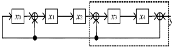
Fig.1 CRC architecture for G(y) = 1 + y + y^3 + y^5 .
