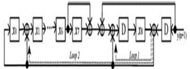
Fig.7 two-level CRC architecture for G(y) = 1 + y + y^8 + y^9 .
