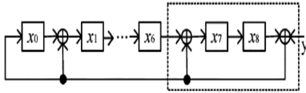
Fig.8. CRC architecture for G(y) = 1 + y + y^8 + y^9 .
