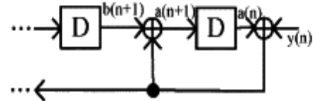
Fig.5 loop bound of 2T_{XOR} .
