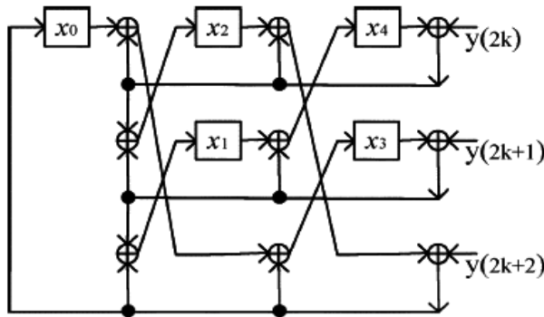
Fig.3 Three-parallel CRC architecture for G(y) = 1 + y + y^3 + y^5 .
