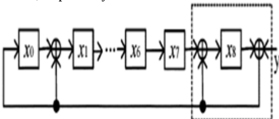
Fig.4. CRC architecture for G(y) = 1 + y + y^8 + y^9 .
