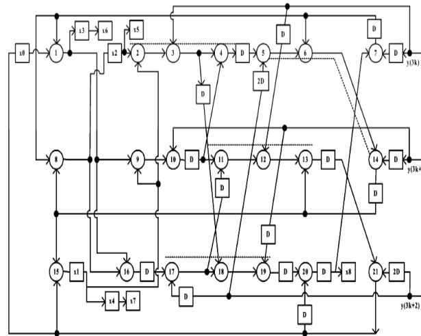
Fig.14. Retimed Three-Parallel CRC Architecture for fig.12(c).
