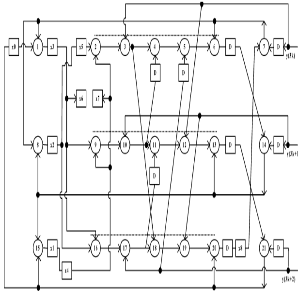
Fig.13.three-parallel CRC architecture for 12(c). after unfolding.
