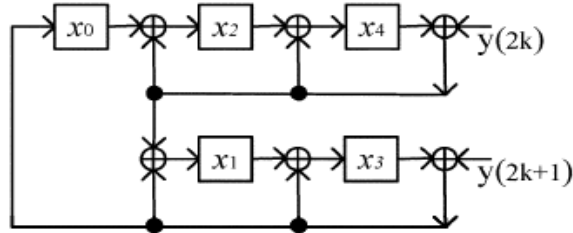
Fig.2 two-parallel CRC architecture for G(y) = 1 + y + y^3 + y^5 .
