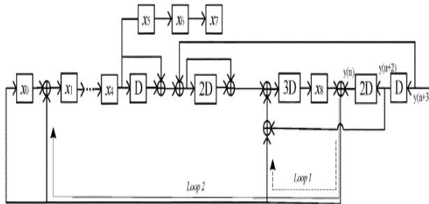
Fig.15.Further Improved Four-Level Pipelined CRC Architecture for G(y) = 1 + y + y^8 + y^9 .
