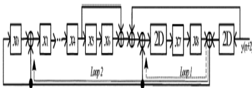
Fig.11. Four-Level Pipelined CRC Architecture For G(y) = 1 + y + y^7 + y^9 .
