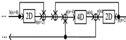
Fig.10. pipelined loop with a loop bound of (1/2)T_{XOR} .
