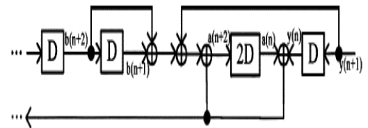
Fig.6 pipelined loop with a loop bound of T_{XOR} .
