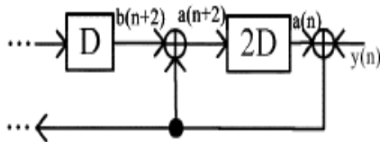
Fig.9. Loop Bound of T_{XOR} .
