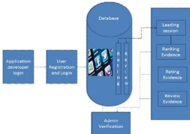
Fig.1.Architecture diagram.
