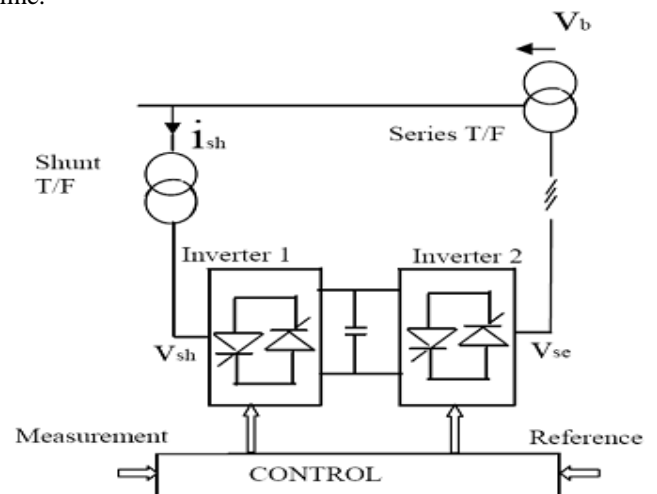
Fig.1. UPFC installed in a transmission line.
