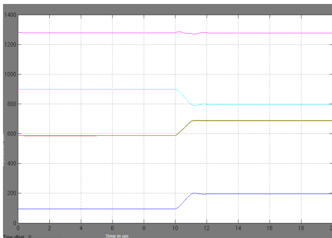
Fig.7. Graphical result by using UPFC.
