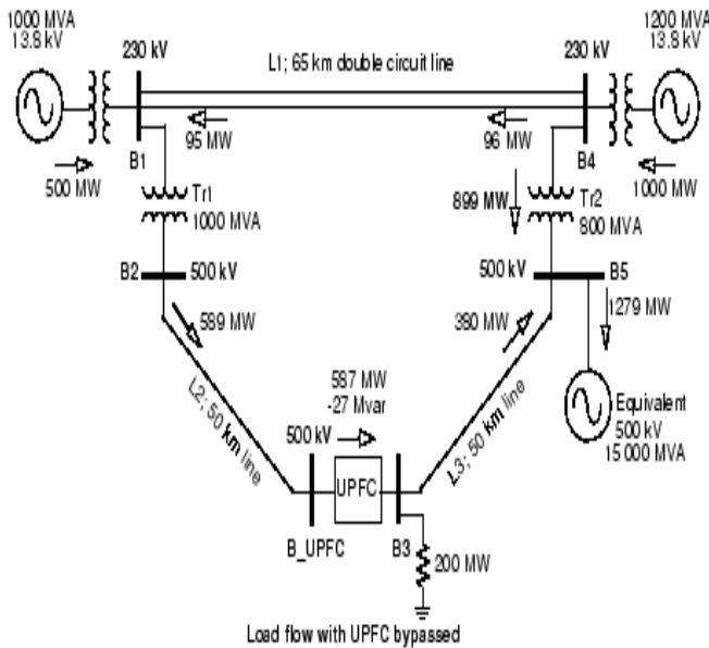
Fig.2. The Single line diagram of a 500kv/230kv transmission system using UPFC.
