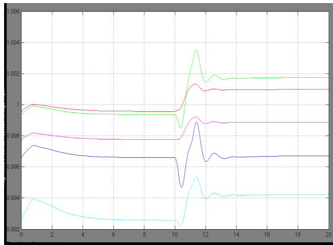
Fig.6. Graphical result by using UPFC.
