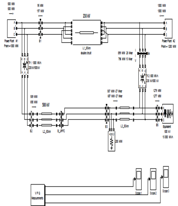
Fig.3. MATLAB Simulink model of single line diagram transmission system using UPFC.
