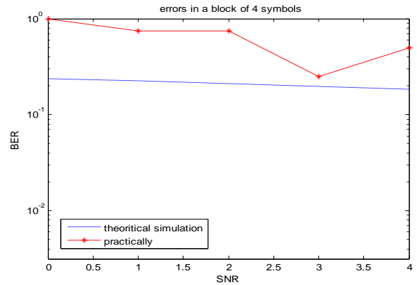
Fig7. Performance of SNR Vs BER at 4-symbols
