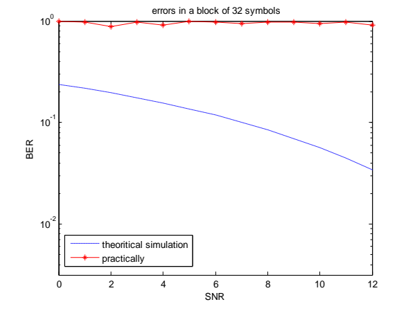
Fig10. Performance of SNR Vs BER at 32-symbols
