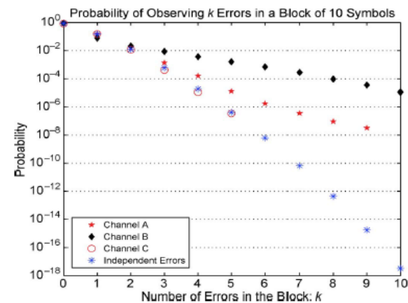
Fig. 4. Joint error statistics for the channels
