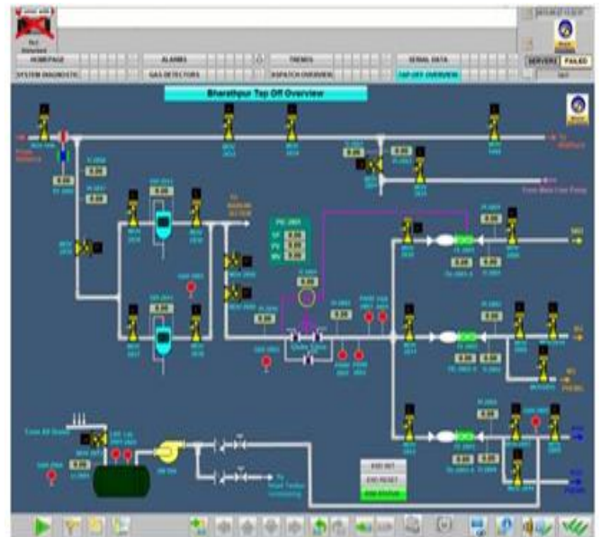
Fig4. Sample Project Screen of Oil Pipeline.
