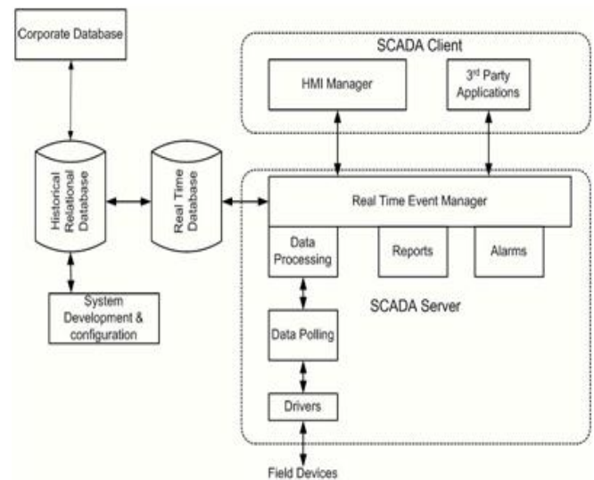
Fig2. High-Level SCADA Host Software Architecture.
