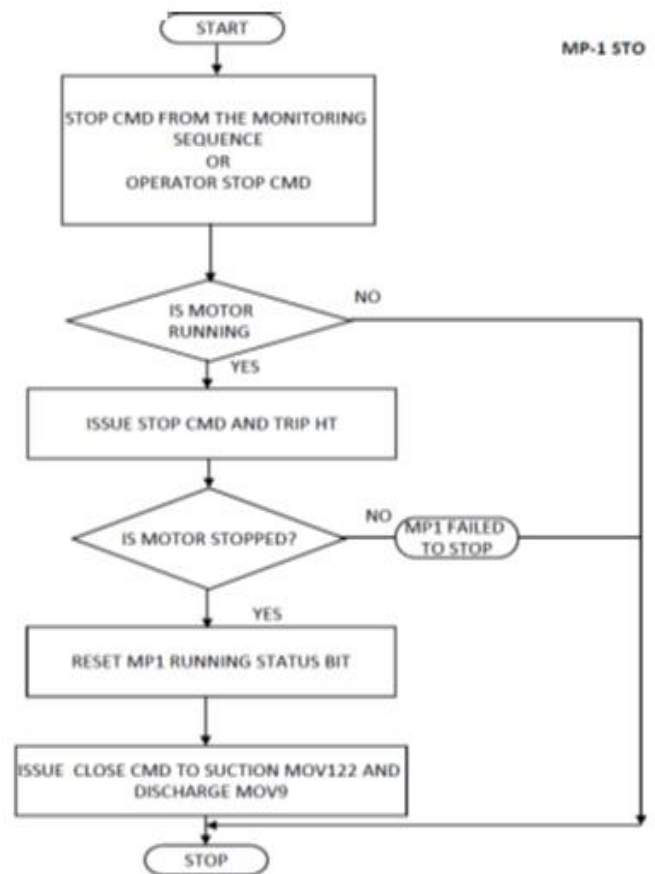
Fig6. Sample Flow Charts for Main Pump Stop Sequence.
