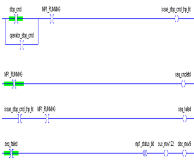
Fig7. Sample Ladder Diagram for Main Pump Stop Sequence.
