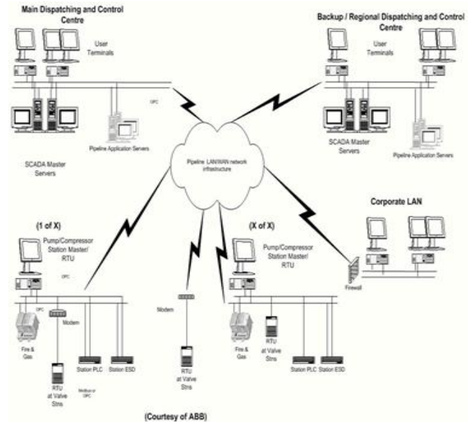
Fig1. Typical SCADA Architecture.
