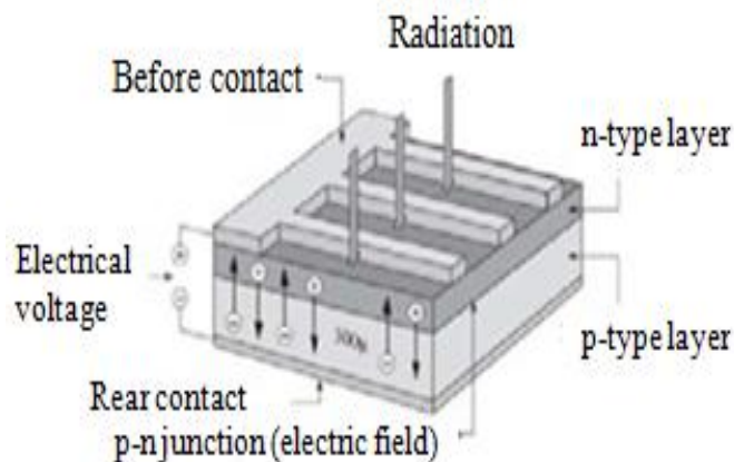
Fig.1. Solar Photovoltaic Cells.
