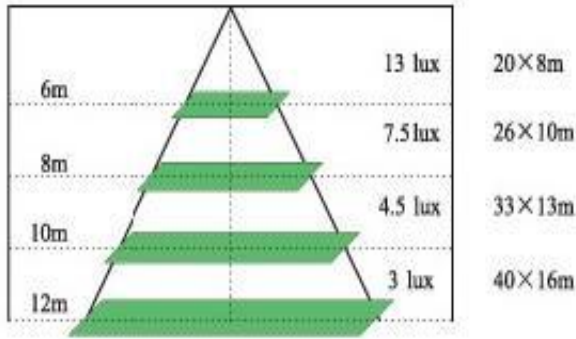
Fig.4. Area of illumination distribution.
