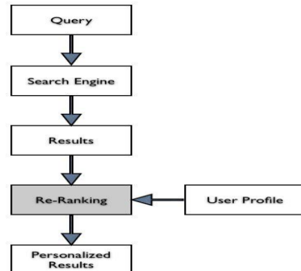
Fig1. Reranking Process.
