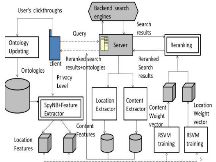
Fig1. OBPMSE Client-Server Architecture
