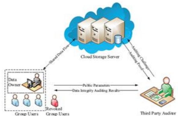
Fig.1. The cloud storage model.
