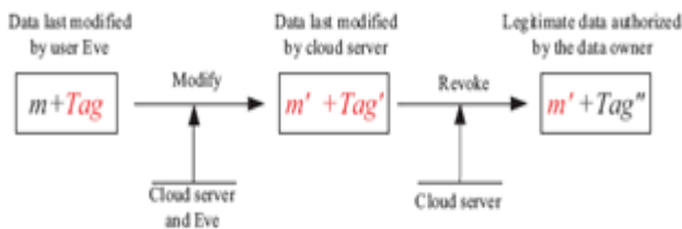
Fig.2 Security problem of server proxy group user revocation.
