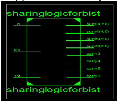
Fig.9. Schematic view.
