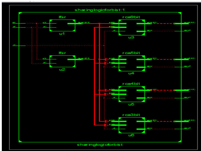
Fig.10. RTL Schematic view.
