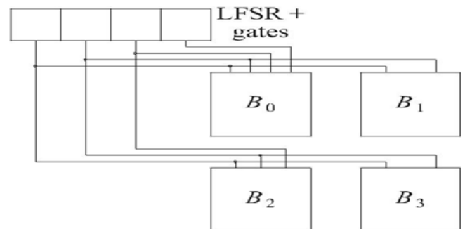
Fig.7. Test Generation Logic for Group.
