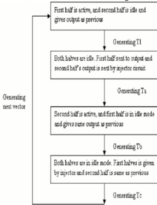
Fig.6. Proposed algorithm for low power LFSR.
