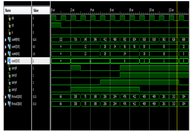
Fig.11. Waveform.
