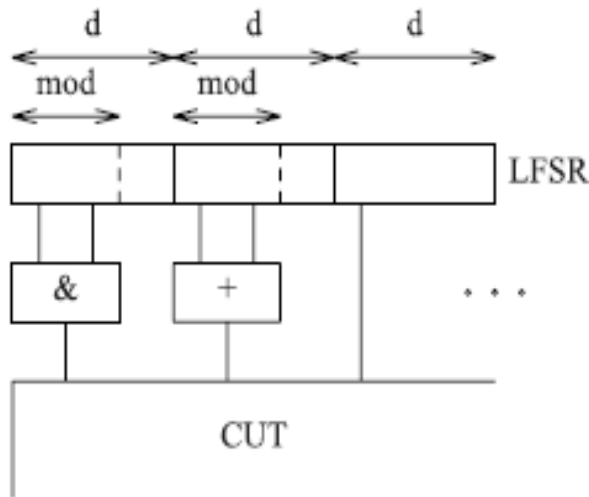
Fig.2. Test Generation Logic.
