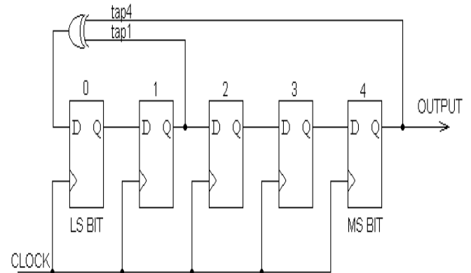
Fig.4. The Architecture for LFSR.
