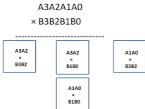
Fig.5. A sample representation of 4-bit Vedic multiplication.
