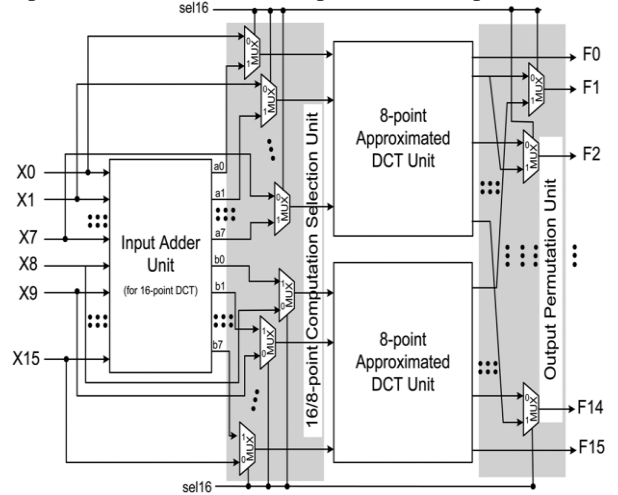
Fig.3. Reconfigurable Architecture for DCT of lengths n=8 & 16.
