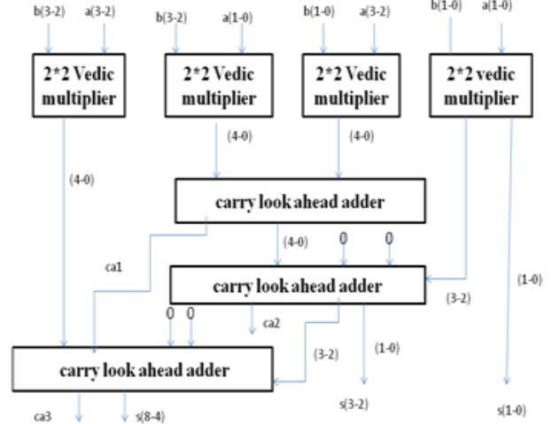
Fig.6. Block diagram for 4-bit Vedic multiplication.
