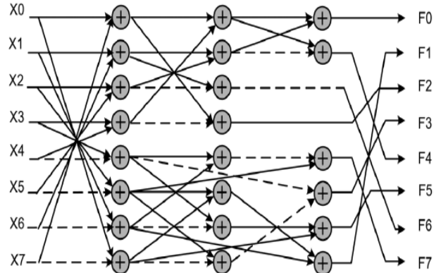
Fig.1. Signal Flow Graph (sfg) of (c8).
