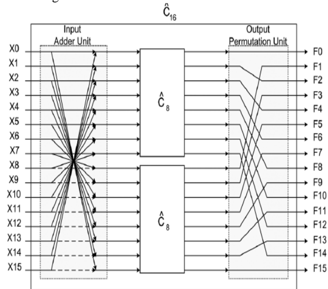
Fig.2. Block diagram of approximation of DCT for n=16.
