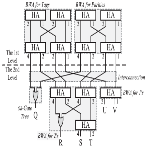
Fig.7. First and second level circuits for a (8, 4) code.
