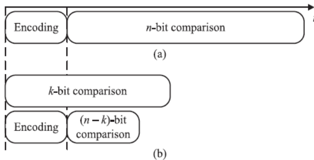
Fig.3. Timing diagram of the tag match in (a) direct compare method and (b) proposed architecture.
