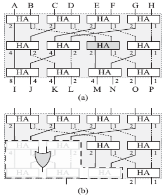
Fig. 6. Proposed BWA. (a) General structure and (b) new structure revised for the matching of ECC-protected data. Note: sum-bit lines are dotted for visibility.
