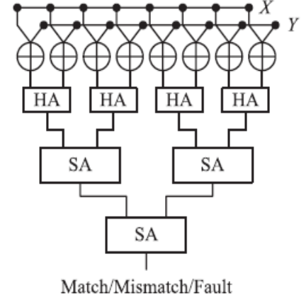
Fig.2. SA based Architecture supporting the direct compare method.
