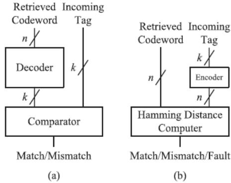
Fig.1. (a) Decode-and-compare architecture and (b) encode-and-compare architecture.
