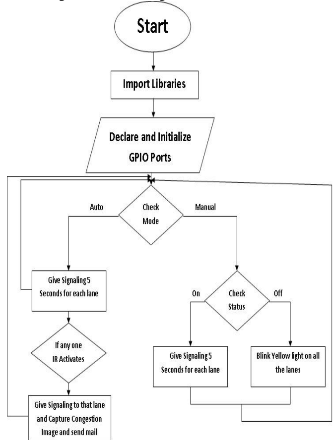
Fig.5. Flow chart of Proposed System.
