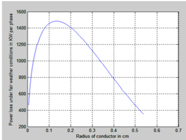
Fig.4. power loss versus size of the conductor.
