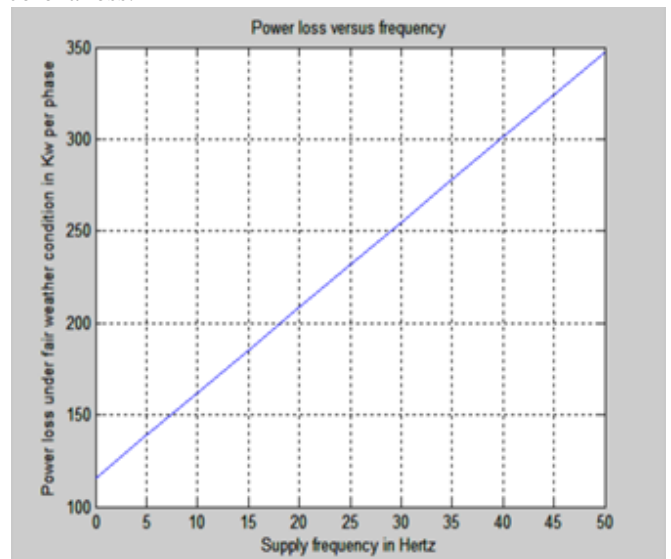
Fig.3. power loss versus frequency.
