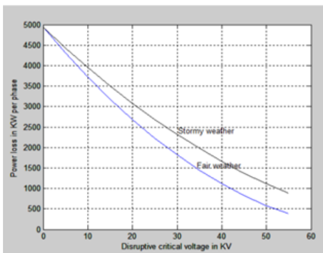
Fig.6. power loss under stormy and fair weather conditions.
