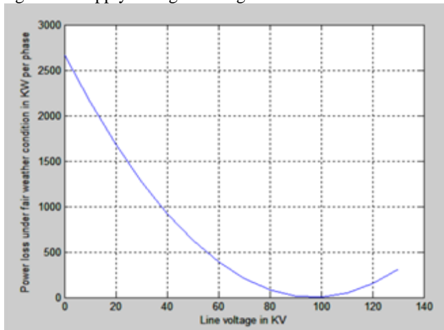
Fig.5. corona loss versus the line voltage.
