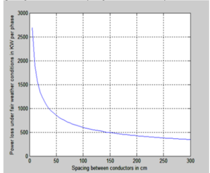
Fig.2. power loss due to corona loss versus the spacing between conductors.
