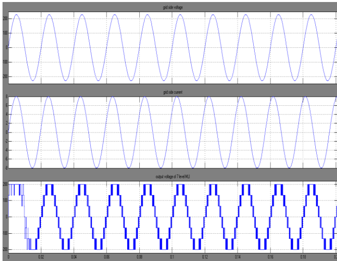
Fig.9. simulation results for the ac side of the seven-level inverter: (a) grid voltage, (b) inverter current (c) output voltage of seven-level inverter.
