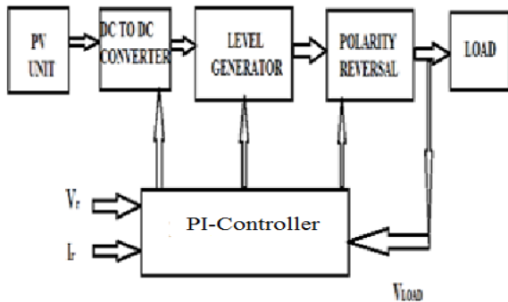
Fig.1. Block Diagram of Proposed Solar Power Generation System.
