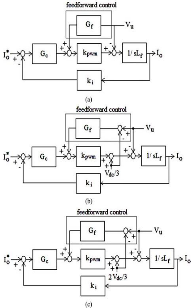
Fig 6. Model of the seven-level inverter under different range of utility voltage, (a) in the range of smaller than V_{dc}/3 , (b) in the range of (V_{dc}/3, 2V_{dc}/3) , (c) in the range of higher than 2V_{dc}/3 .
