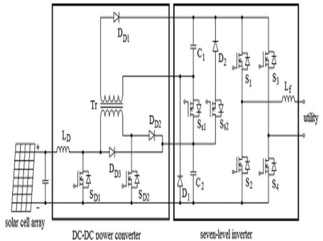
Fig.2. Configuration of the proposed solar power generation system.
