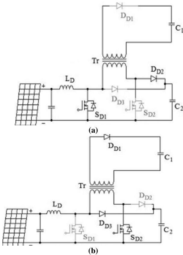
Fig.3. Operation of dc-dc power converter: (a) S_{D1} is on and (b) S_{D1} is off.
