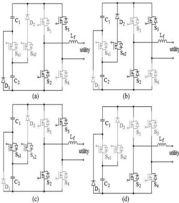
Fig.5. Operation of the seven-level inverter in the negative half cycle:(a) Mode 5, (b) mode 6, (c) mode 7, and (d) mode 8.
