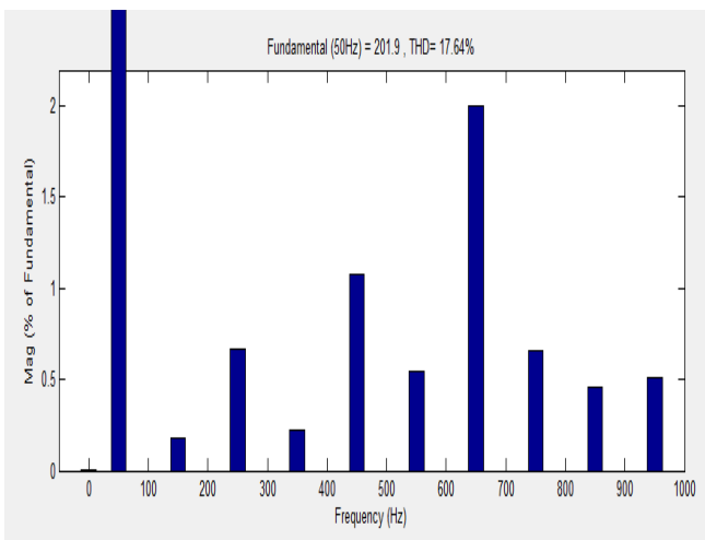
Fig.11. THD analysis for 7 level inverter output Voltage.
