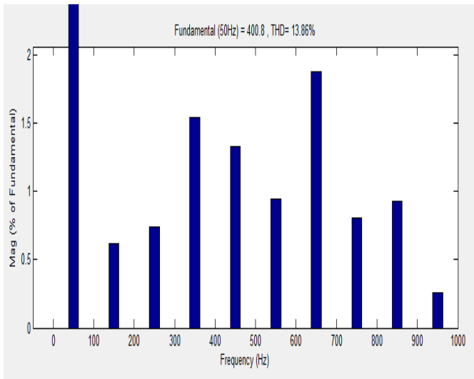
Fig.15. THD analysis shows 13.86% for Nine level output voltage.
