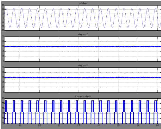
Fig.10. simulation results for seven level (a) grid voltage, (b) voltage of capacitor C1, (c) voltage of capacitor C2, and (d) output voltage of the capacitor selection circuit.
