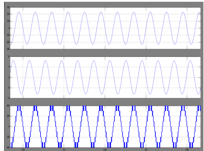
Fig.13. simulation results for the ac side of the nine-level inverter: (a) grid voltage, (b) inverter current (c) output voltage of seven-level inverter.
