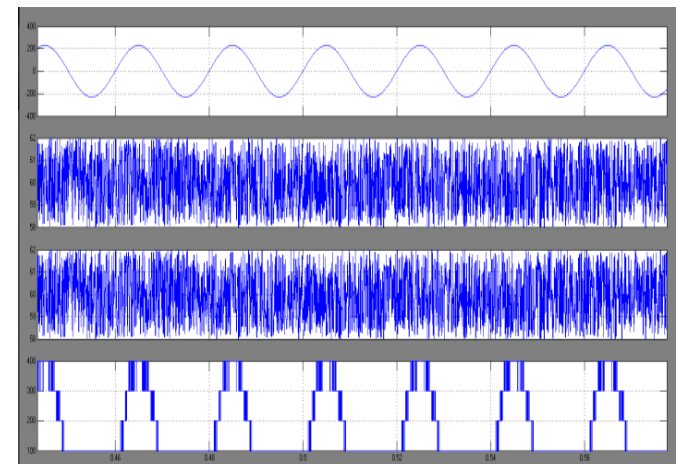
Fig.14. simulation results for nine level (a) grid voltage, (b) voltage of capacitor C1, (c) voltage of capacitor C2, and (d) output voltage of the capacitor selection circuit.
